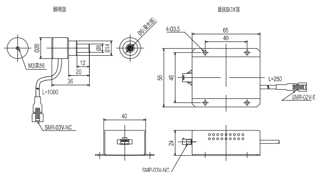
SLDH-A20R SLDH-A20W
